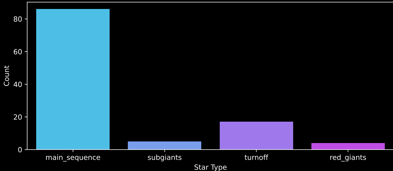
APOGEE DR17 Field: [BOOTES1] Count plot of Star Type
