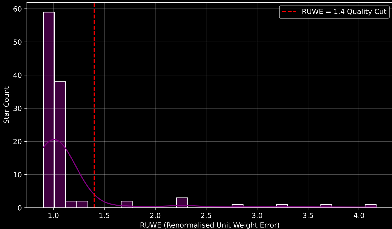
GAPOGEE DR17 Field [BOOTES1] RUWE Distribution (n= 110)
