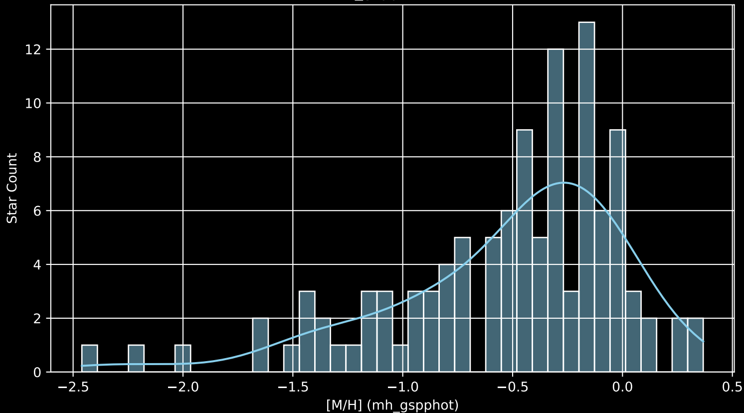
APOGEE DR17 Field: [BOOTES1 [M/H] (mh_gspphot) (n= 112)
