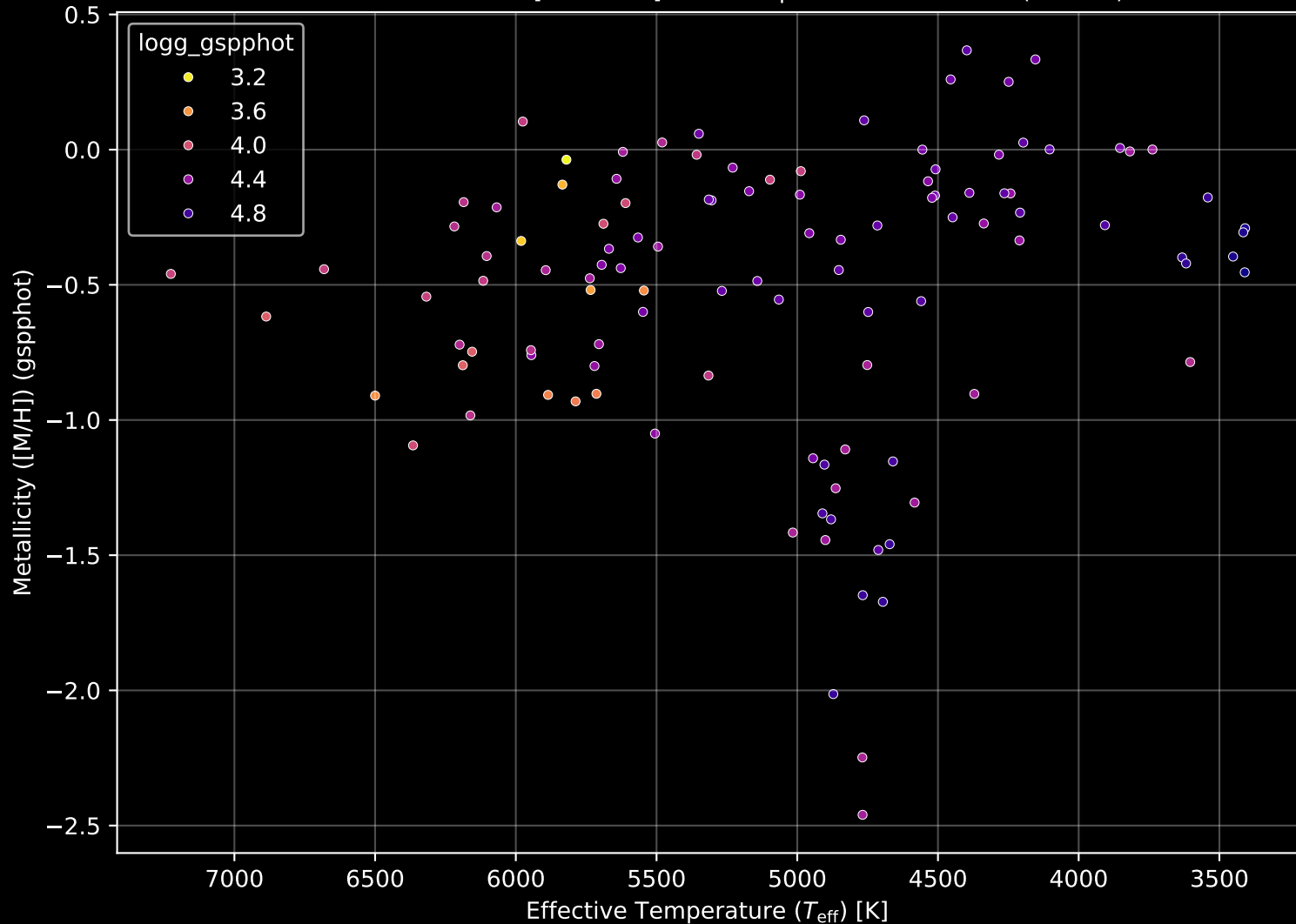
APOGEE DR17 Field: [BOOTES1] Stellar Population Parameters (n= 112)
