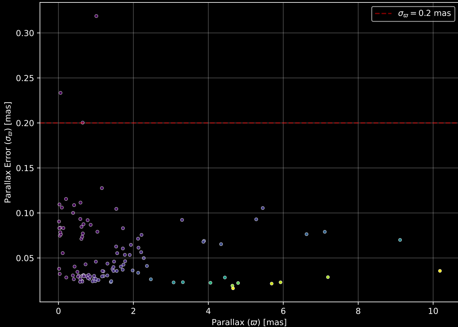
APOGEE DR17 Field: [BOOTES1] Parallax Quality (n= 112)
