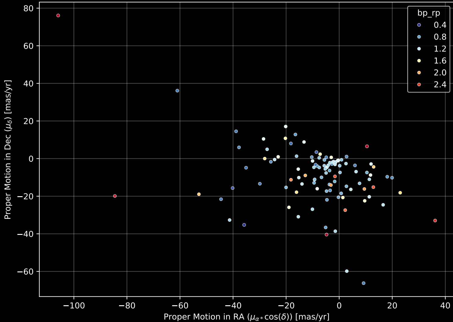
APOGEE DR17 Field: [BOOTES1] Proper Motion Diagram (n= 112)
